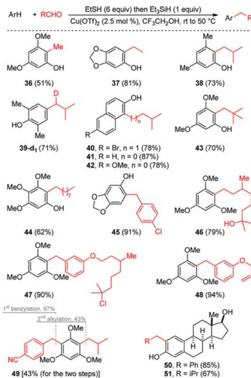
Figure 2. Scope of the reductive alkylation reaction. For the exact reaction conditions, see SI.
