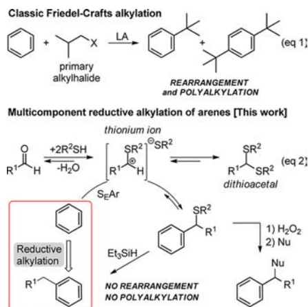
Scheme 1. Classic Friedel–Crafts Alkylation (eq 1), Reductive Alkylation of Arenes (eq 2)
