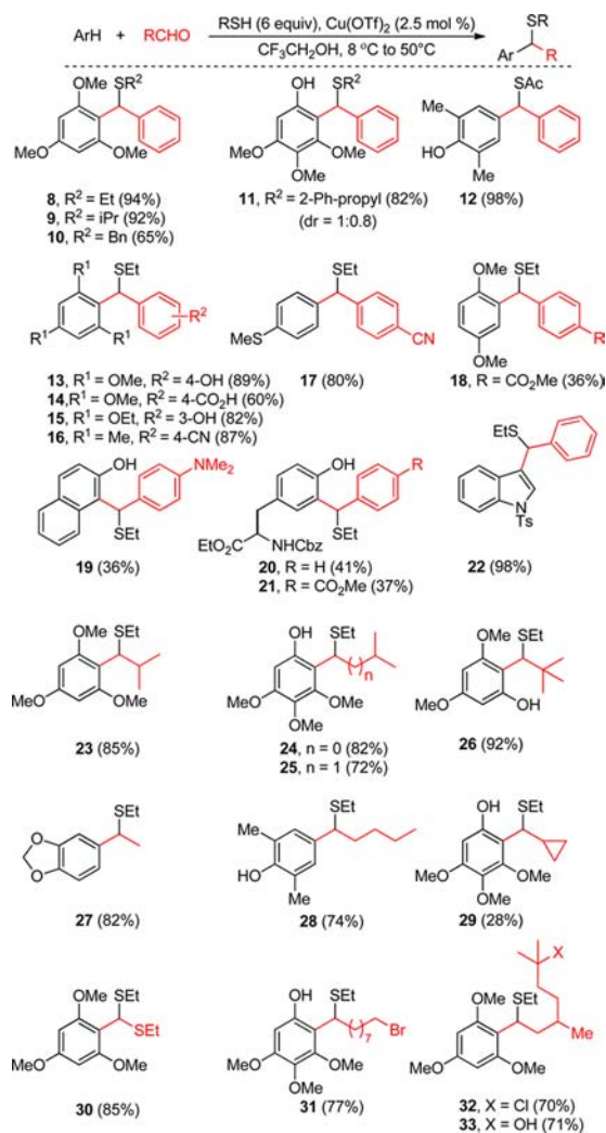
Figure 1. Scope of the thiol-based multicomponent alkylation of arenes. For the exact reaction conditions, see SI.
